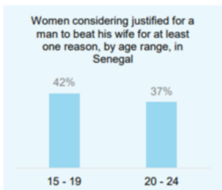
FIGURE 2: DHS, SENEGAL, 2017
