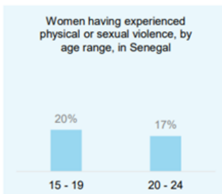
FIGURE 1: DHS, SENEGAL, 2019
